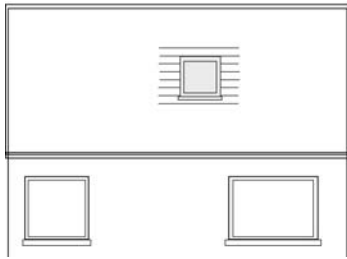
Part Front Elevation Scale 1:50
