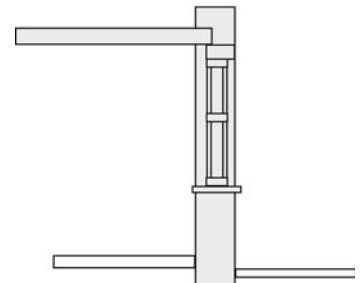
Section Scale 1:50
