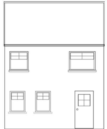
Front elevation Scale 1:50
